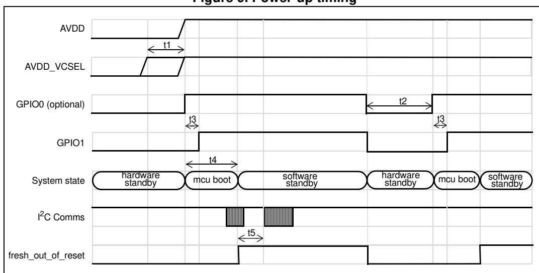
Figure 9. Power-up timing
