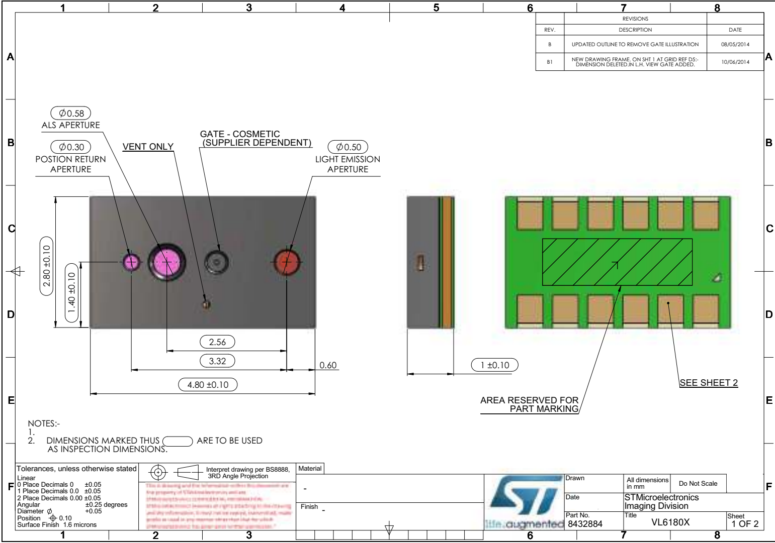
Figure 27. Outline drawing (page 1/2)
